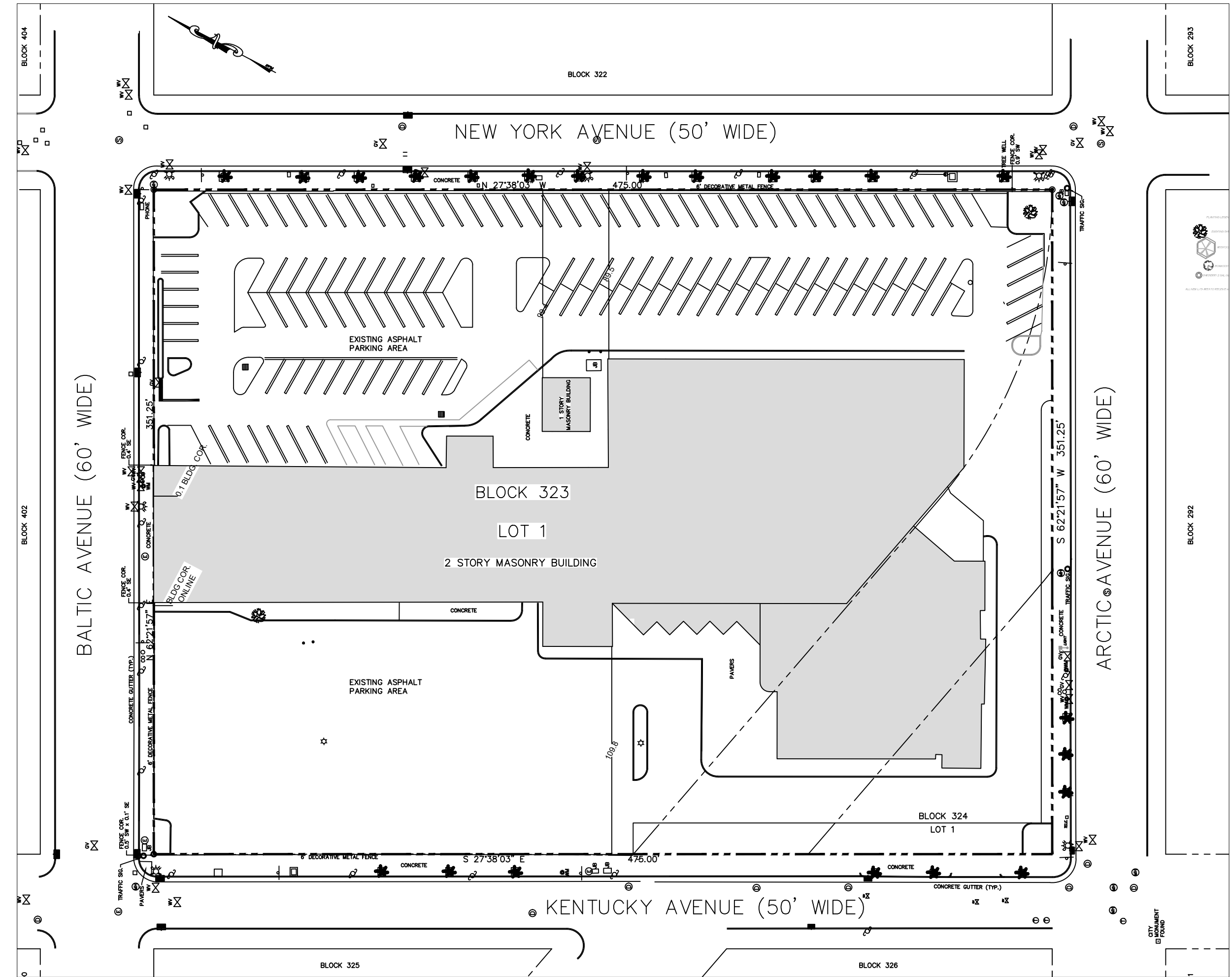
EXISTING CONDITIONS SURVEY SCALE: 1" = 50'
