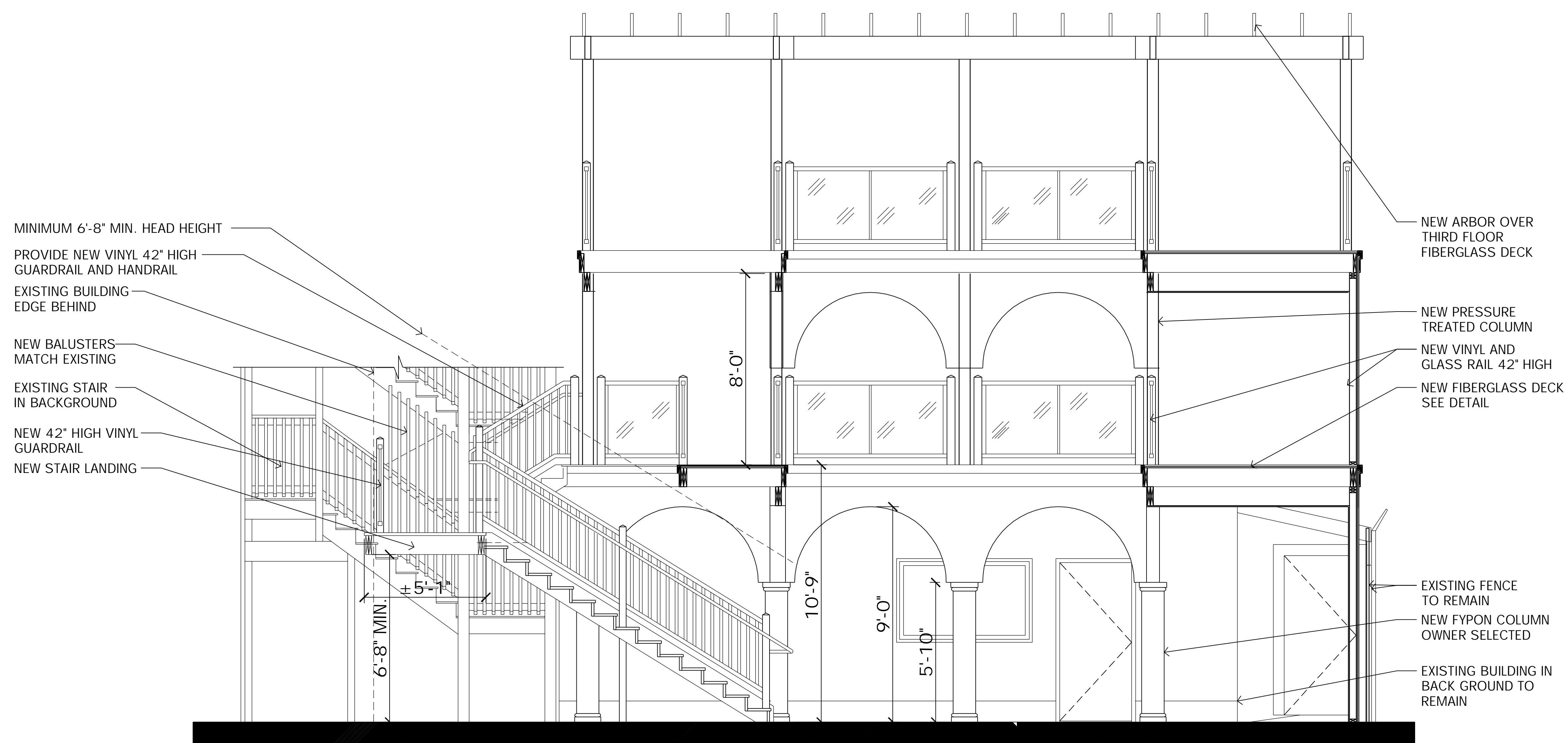
EXTERIOR COURTYARD SECTION / ELEVATION
