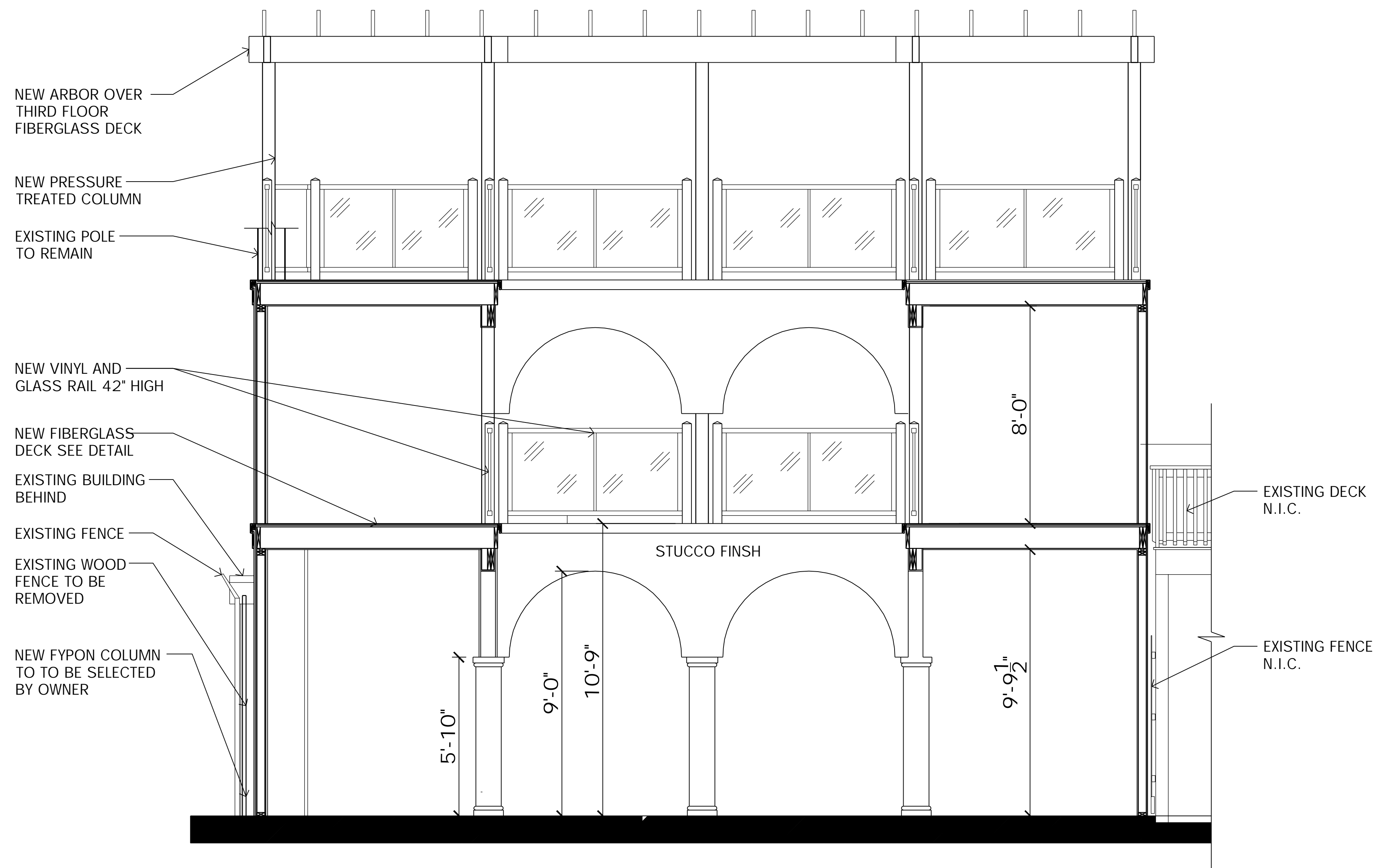
EXTERIOR COURTYARD SECTION / ELEVATION
