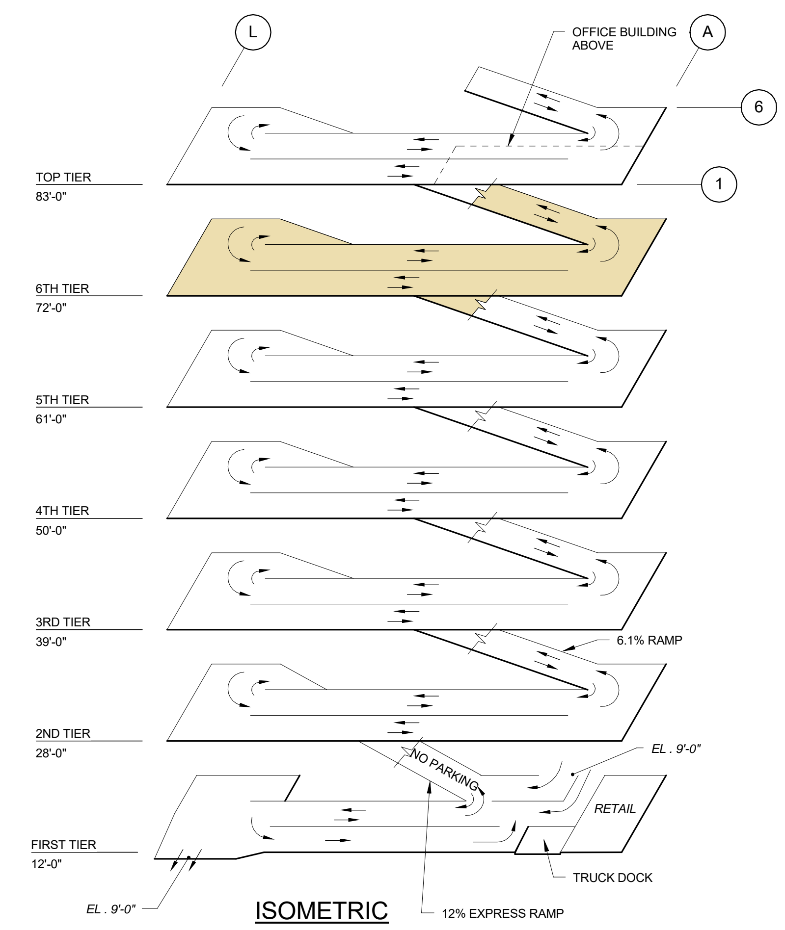
ISOMETRIC
