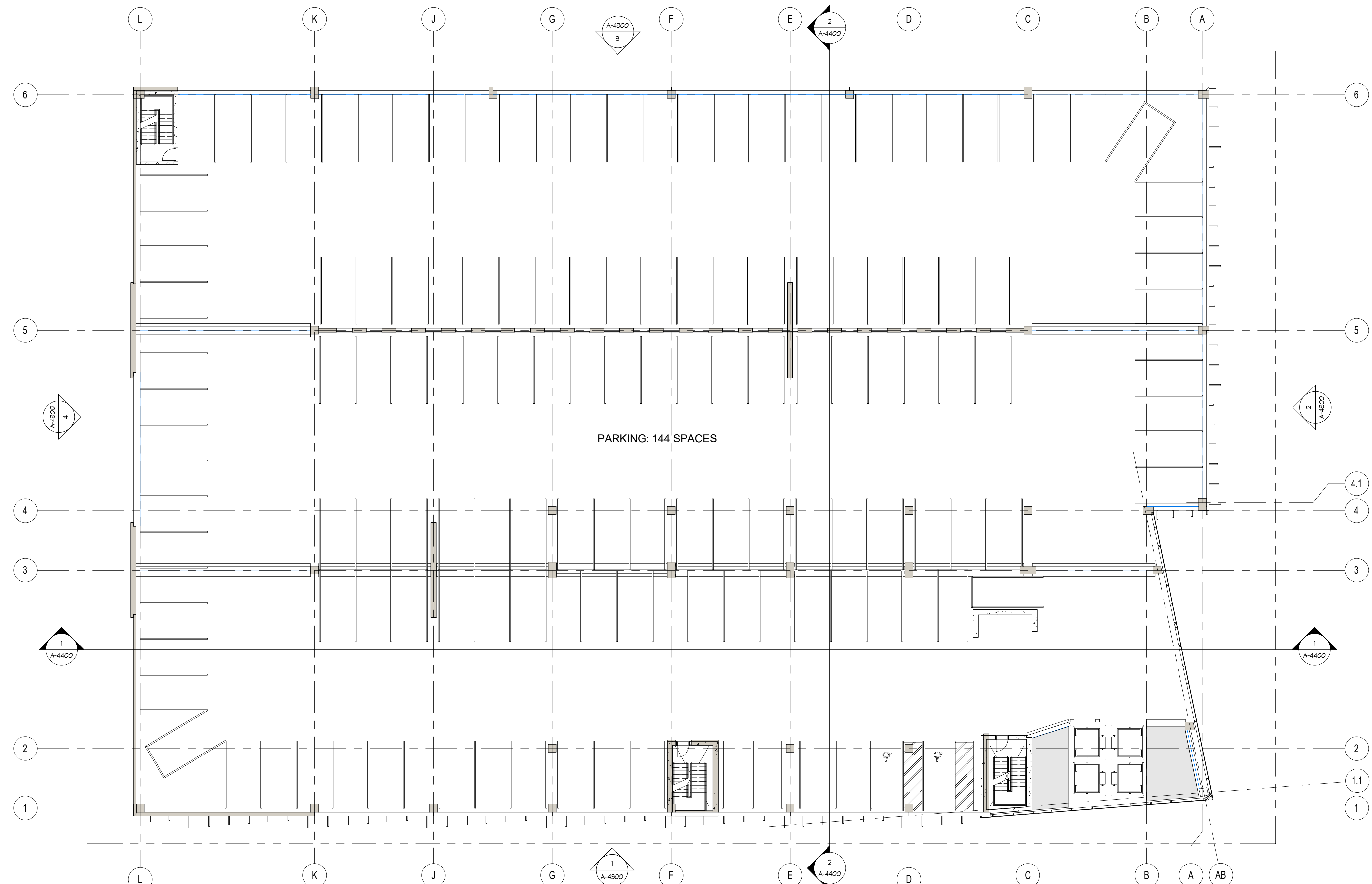
1 FIFTH FLOOR GARAGE PLAN 1/8" = 1'-0"
