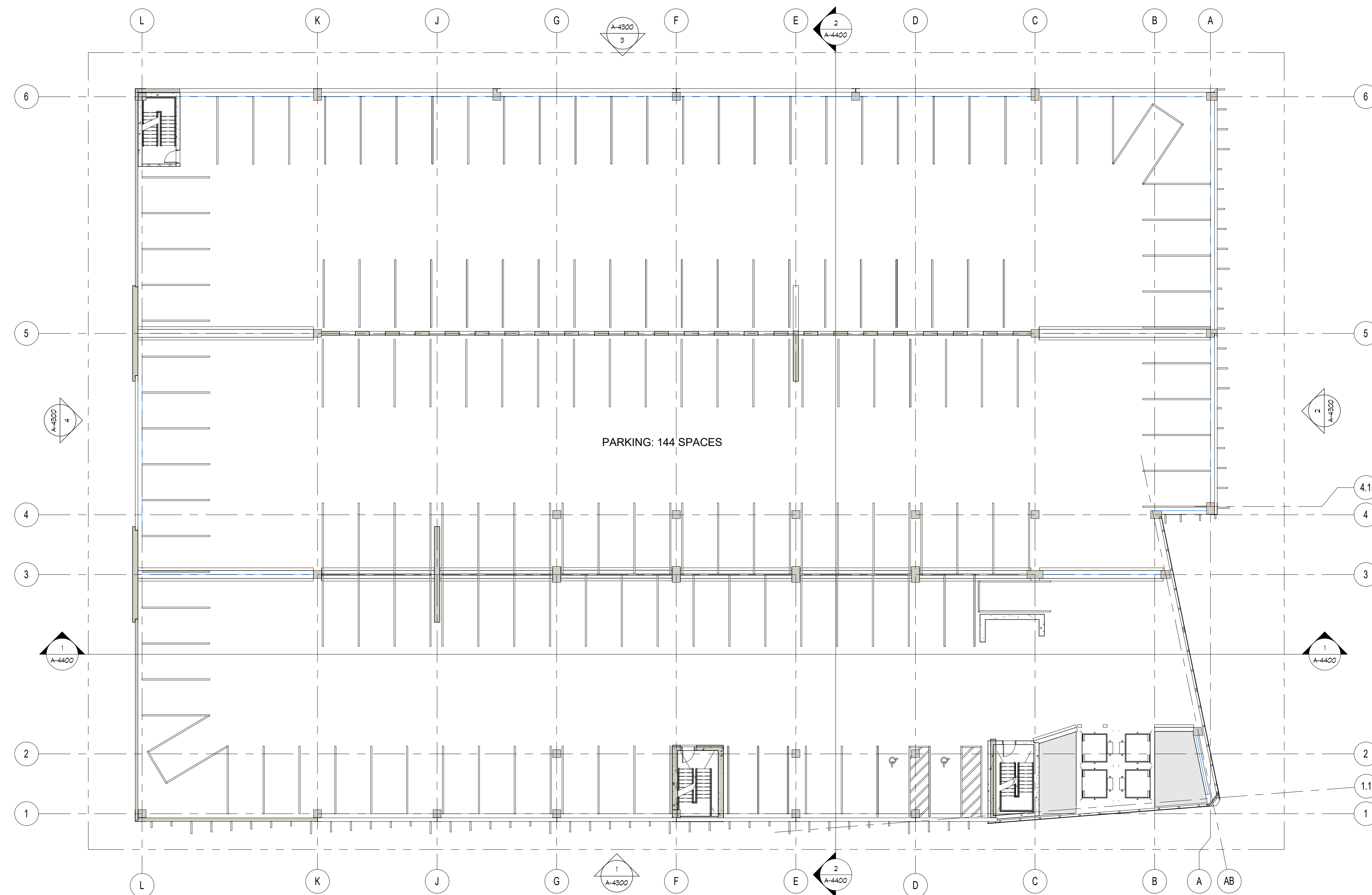
2 SIXTH FLOOR GARAGE PLAN 1/8" = 1'-0"
