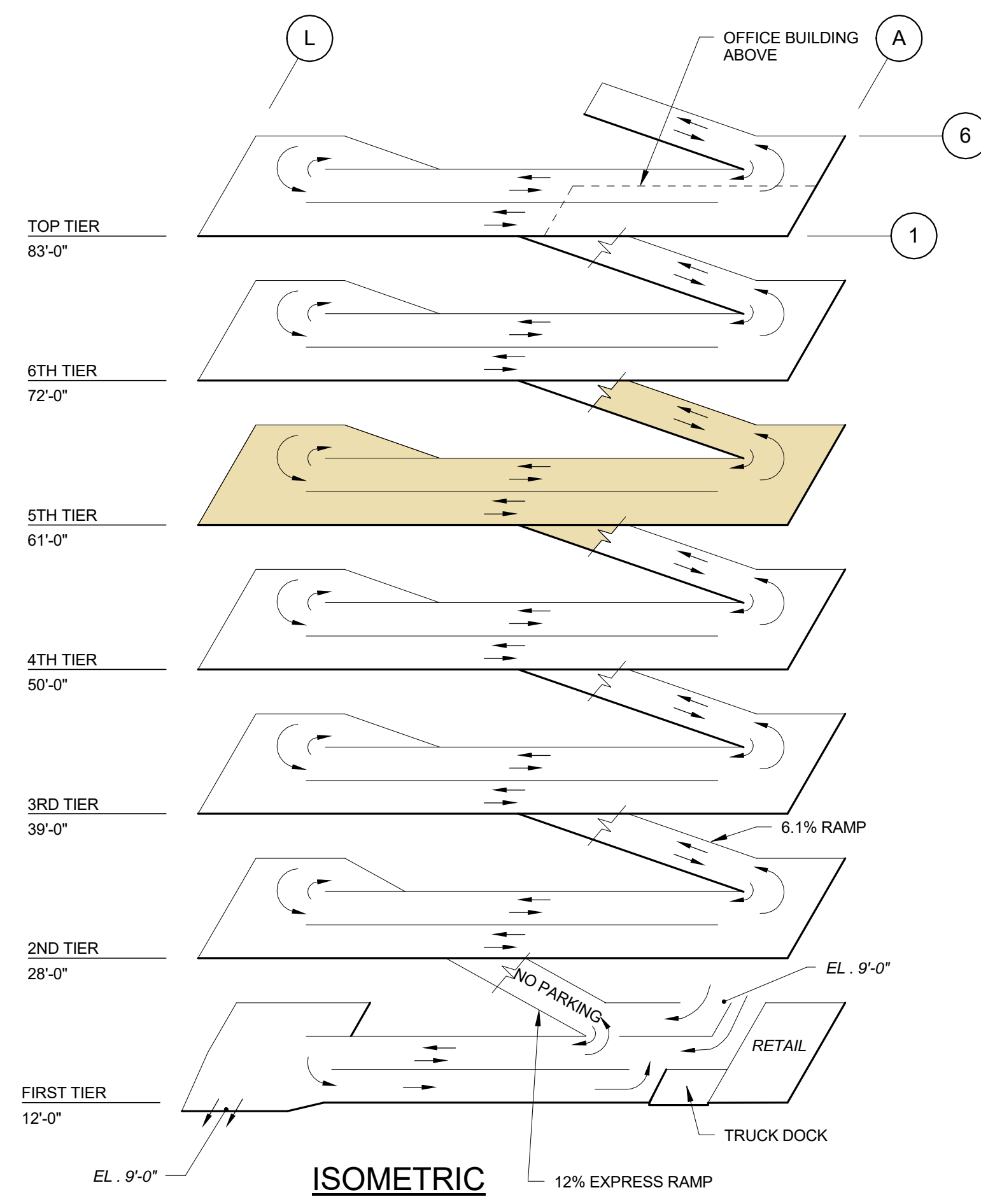
ISOMETRIC
