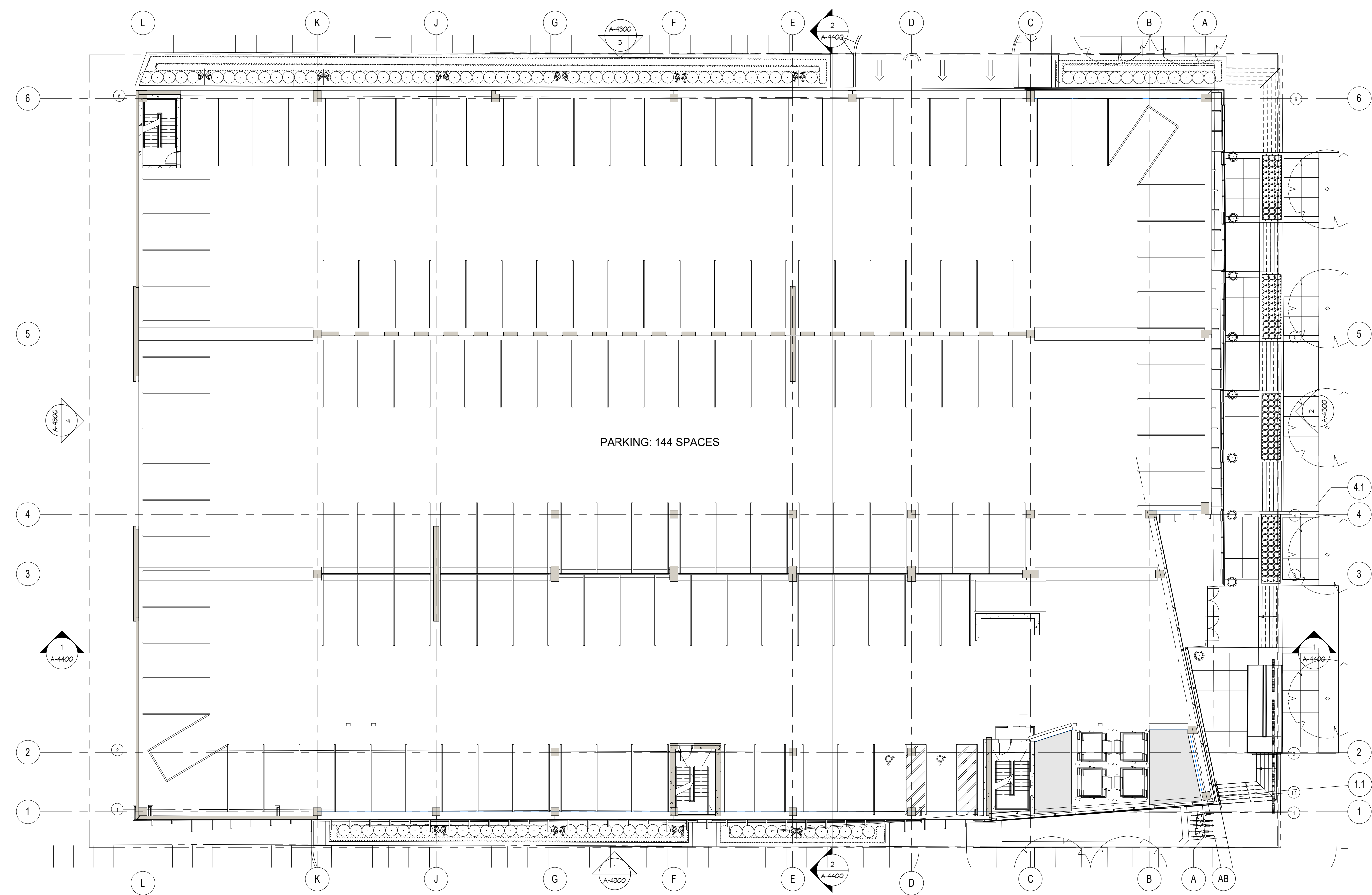
1 THIRD FLOOR GARAGE PLAN 1/8" = 1'-0"
