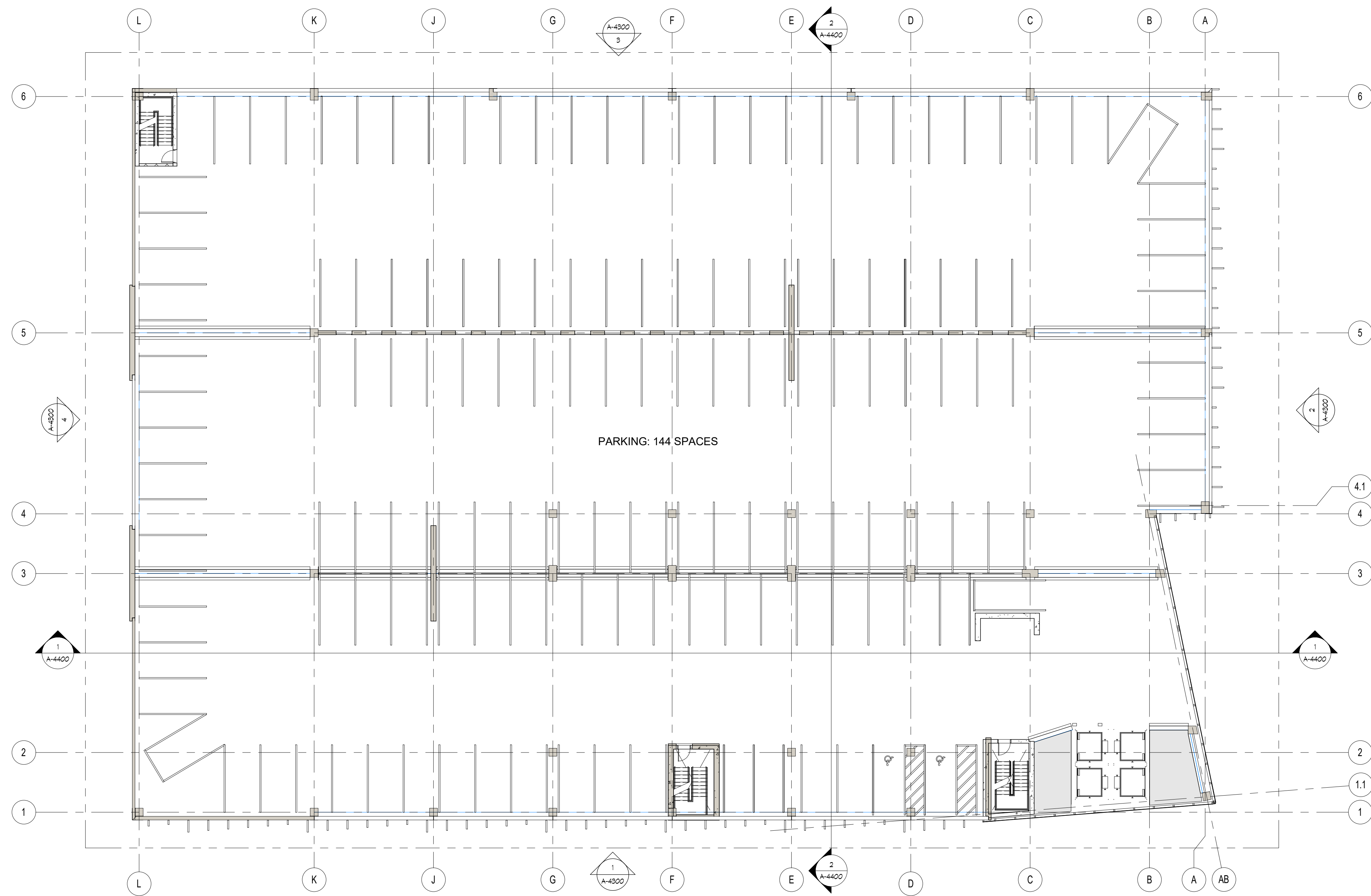
2 FOURTH FLOOR GARAGE PLAN 1/8" = 1'-0"
