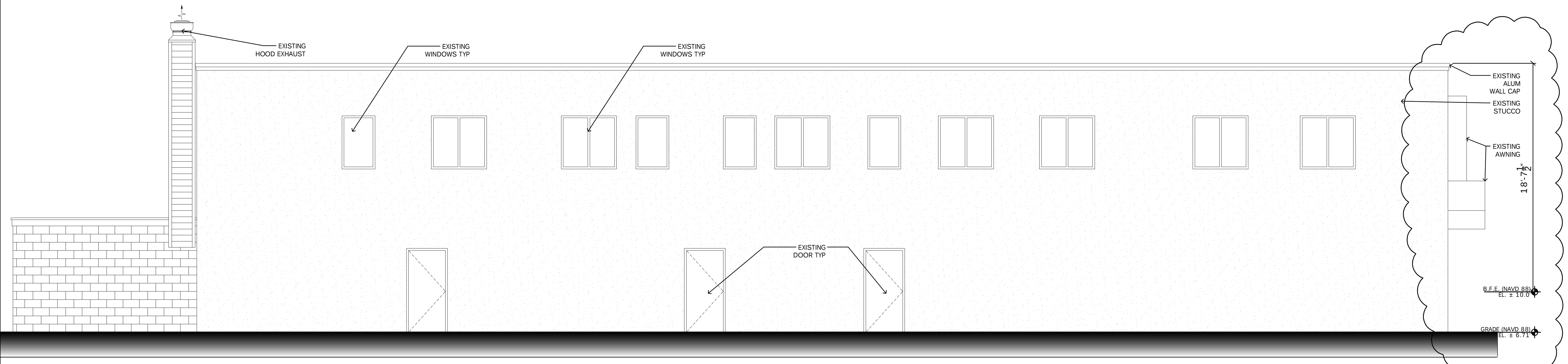
EXISTING SIDE ELEVATION SCALE: 1/4" = 1'-0"
