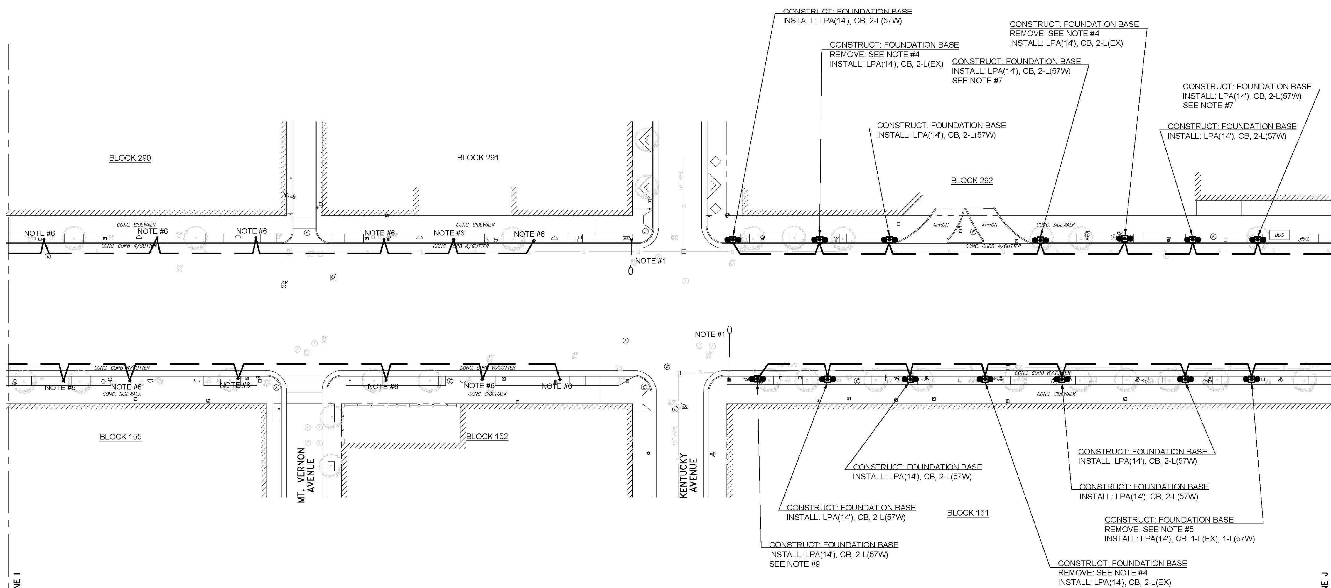
LIGHTING PART PLAN J SCALE: 1" = 30'-0"
