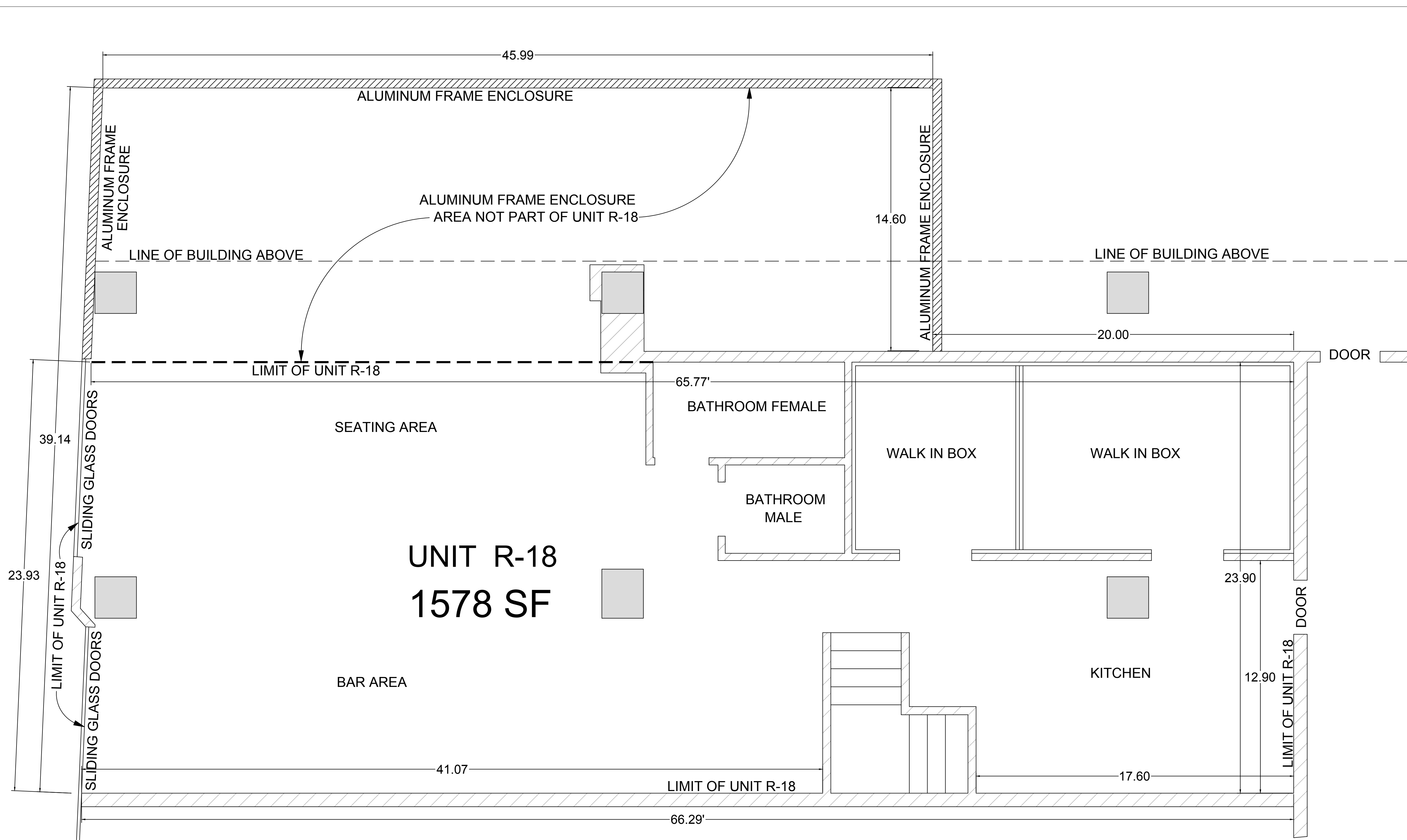
INTERIOR FLOOR PLAN SCALE 1" = 3'
