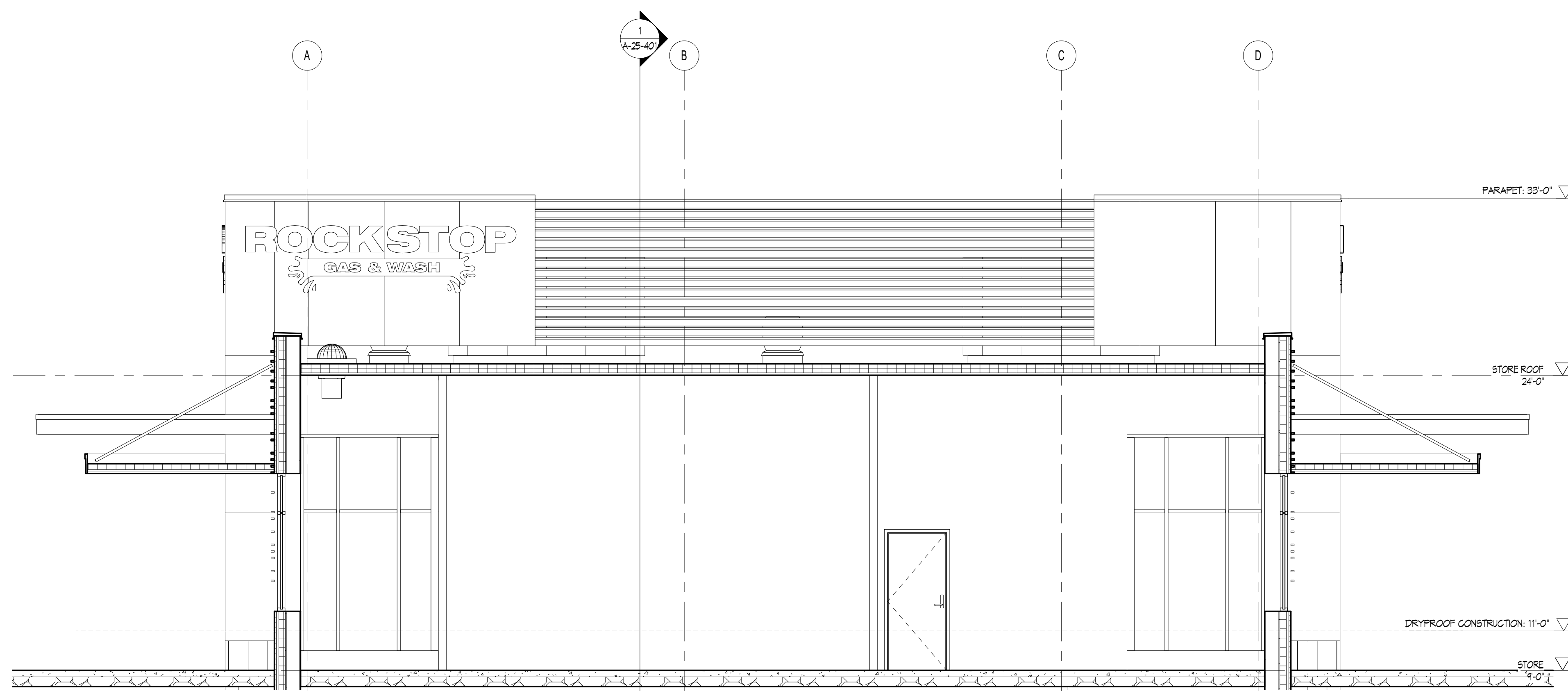
2 BUILDING SECTION - STORE 1/2" = 1'-0"
