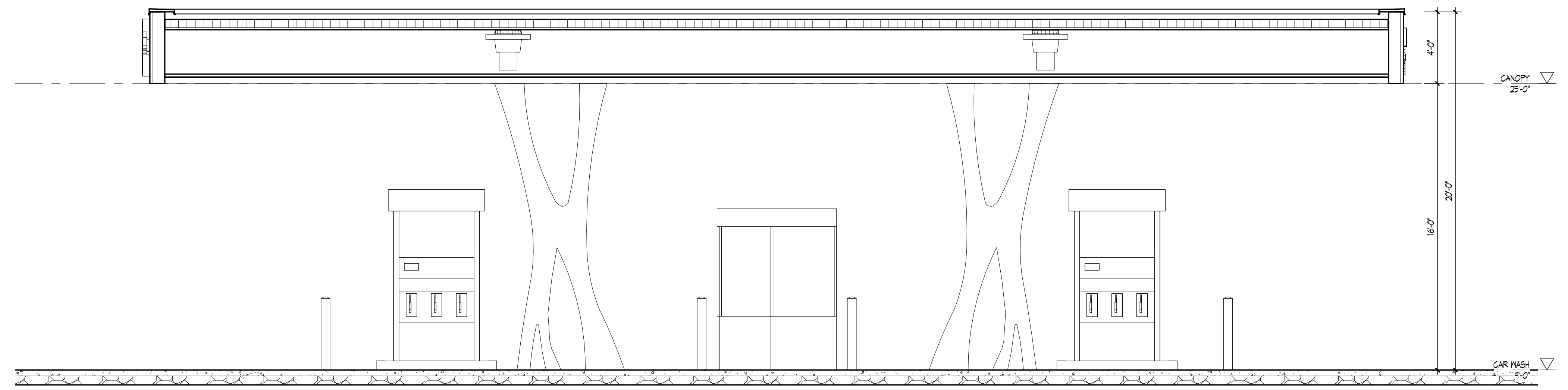
5 BUILDING SECTION - CANOPY 1/4" = 1'-0"
