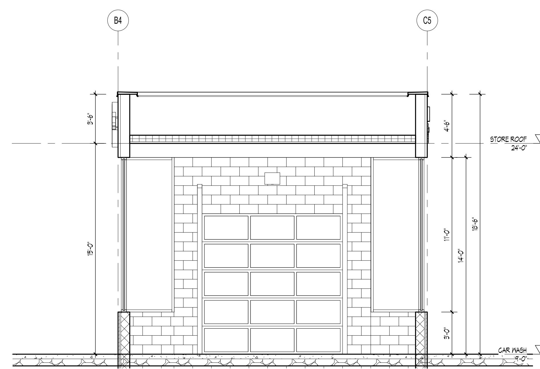
3 BUILDING SECTION - CAR WASH 1/4" = 1'-0"
