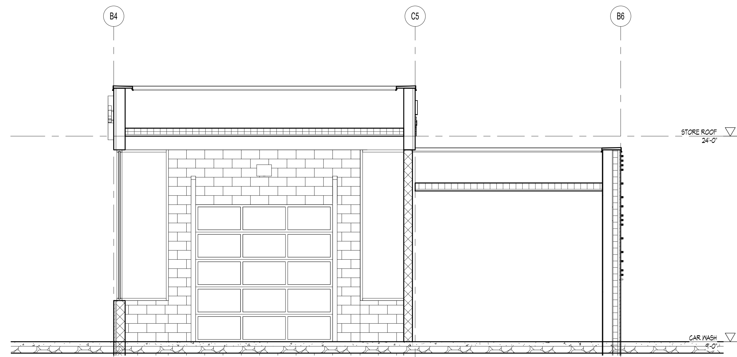
4 BUILDING SECTION - CAR WASH 1/4" = 1'-0"
