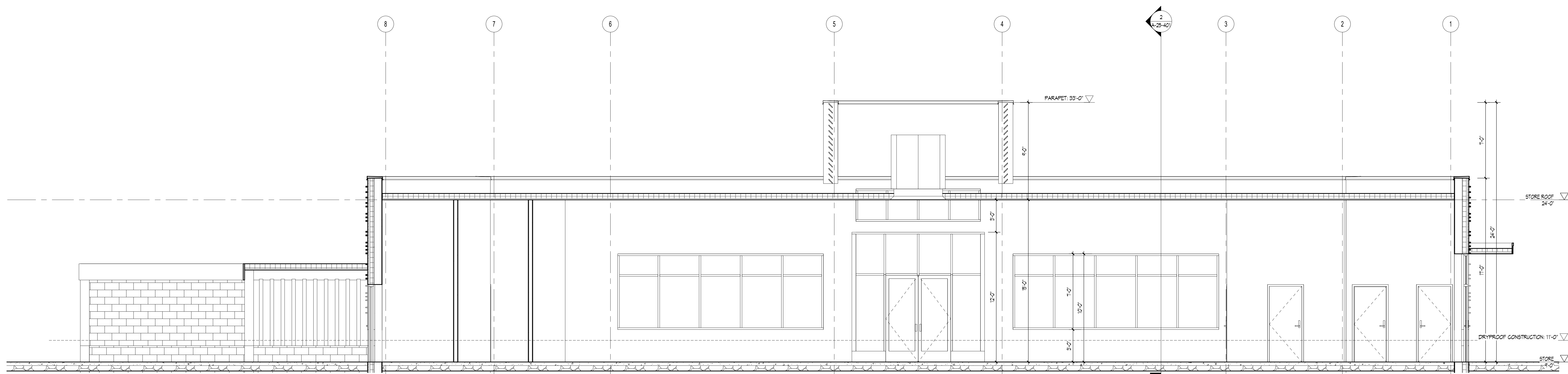
1 BUILDING SECTION - STORE 1/2" = 1'-0"
