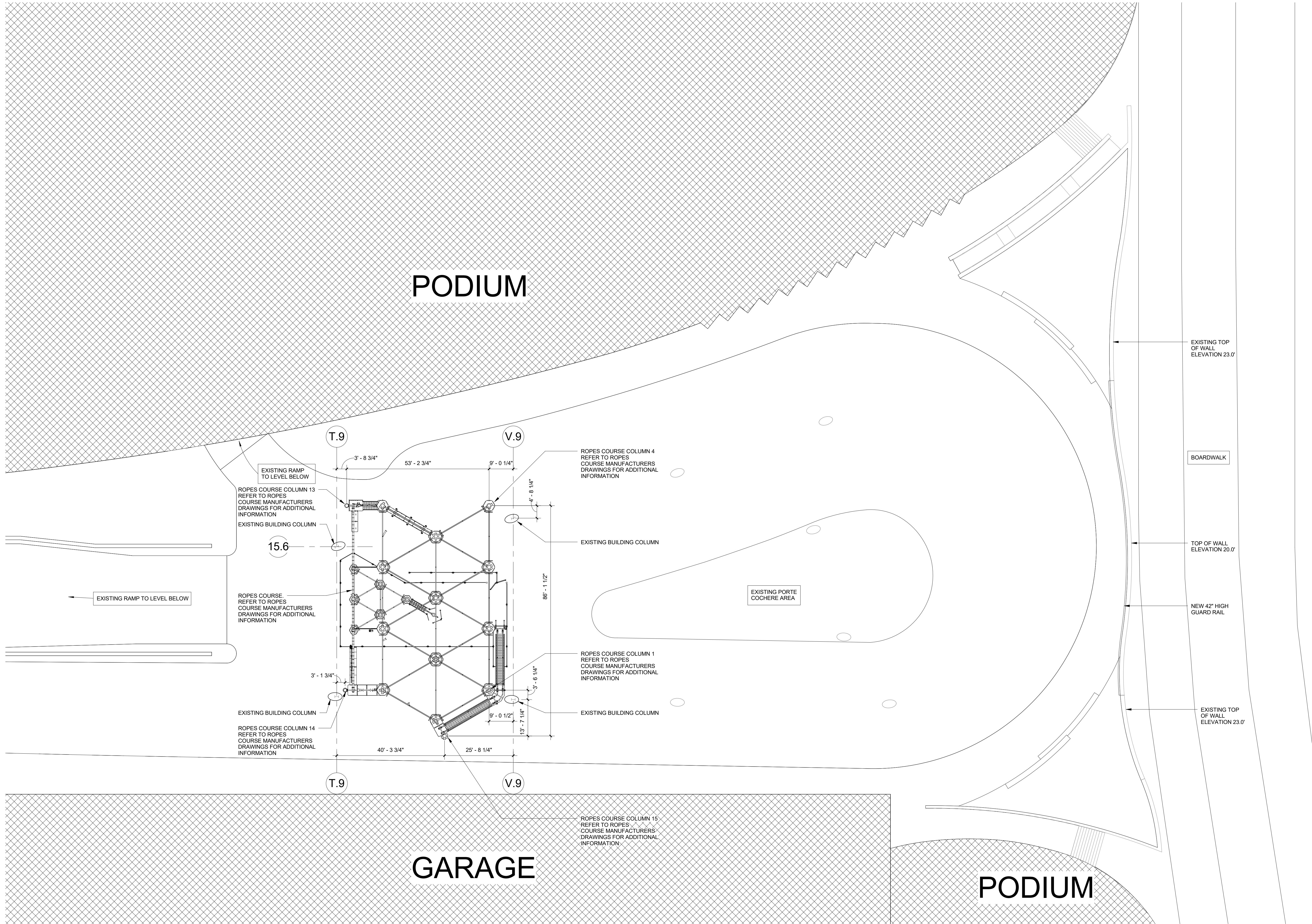
1 ROPES COURSE LOCATION PLAN 1/16" = 1'-0"
