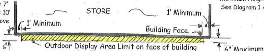
Diagram 3 - PLAN - WITH OPEN STOREFRONT
